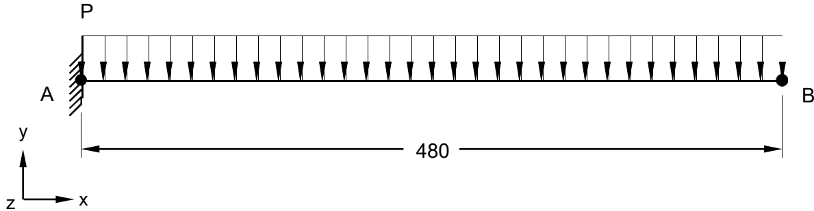
Figure 1. Cantilever Beam with Distributed Load
