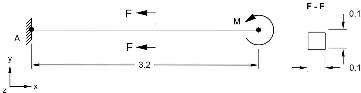
Figure 1. Cantilever Model
