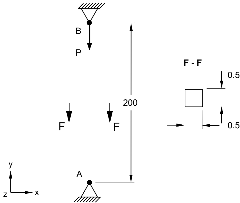
Figure 1. Bar Model
