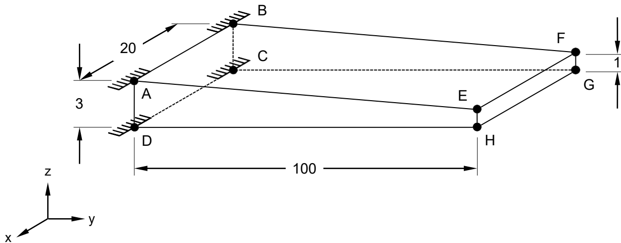
Figure 1. Tapered Solid Model
