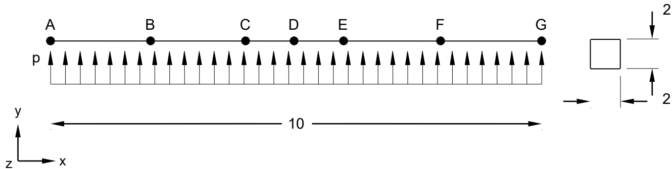
Figure 1. Beam Cross-Section Model
