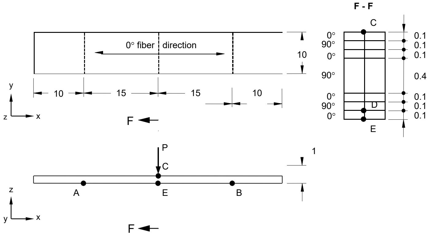
Figure 1. Laminated Strip
