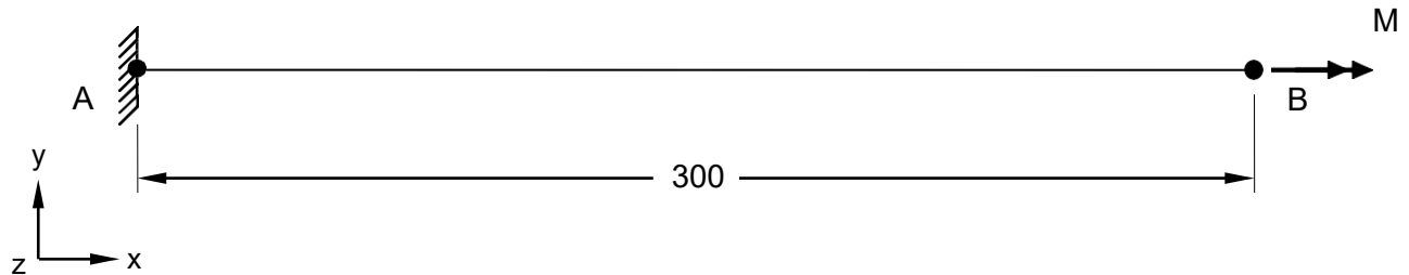
Figure 2. Boundary Conditions
