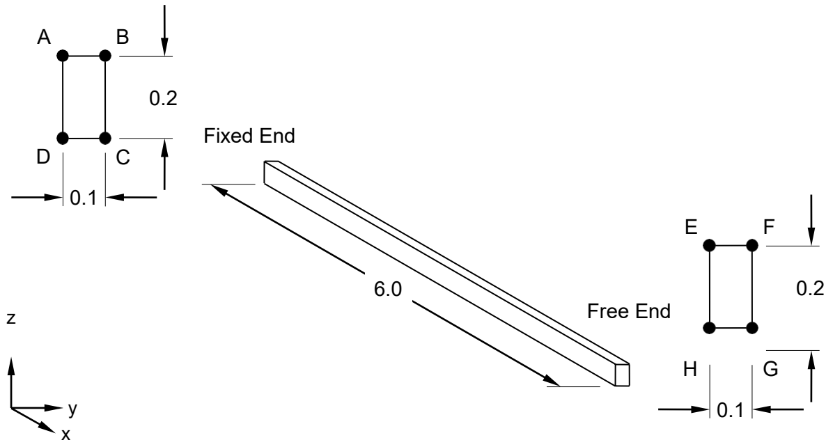
Figure 1. Beam Model
