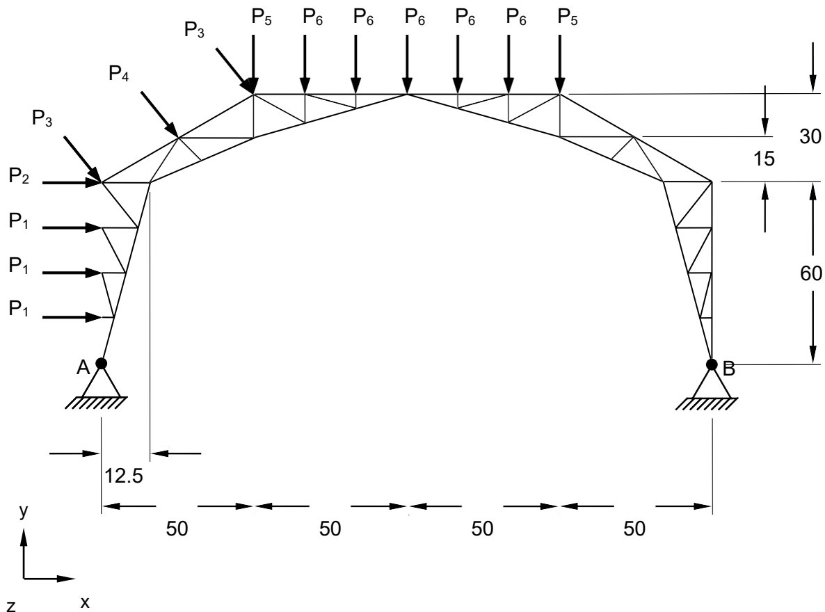
Figure 1. Truss Model
