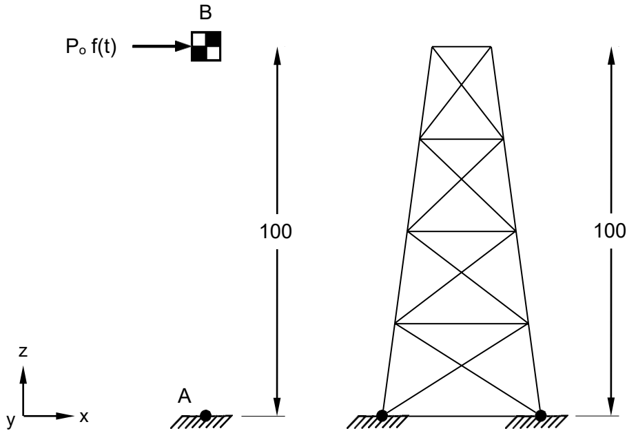
Figure 1. Tower Model
