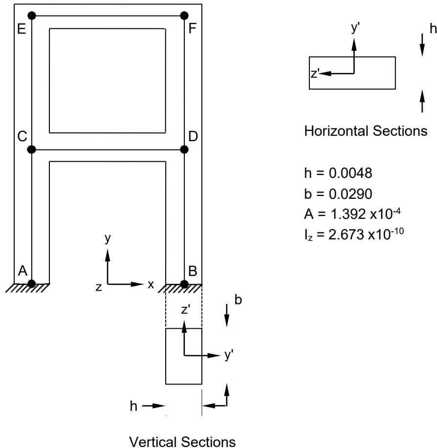
Figure 1. Symmetric Truss
