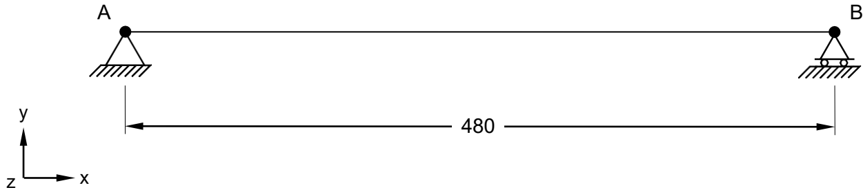
Figure 1. Beam Model
