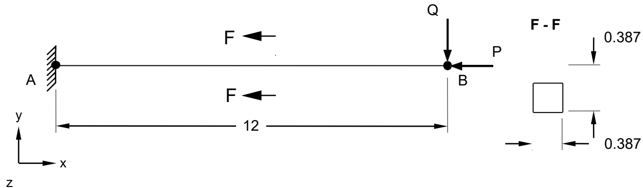
Figure 1. Cantilever Model
