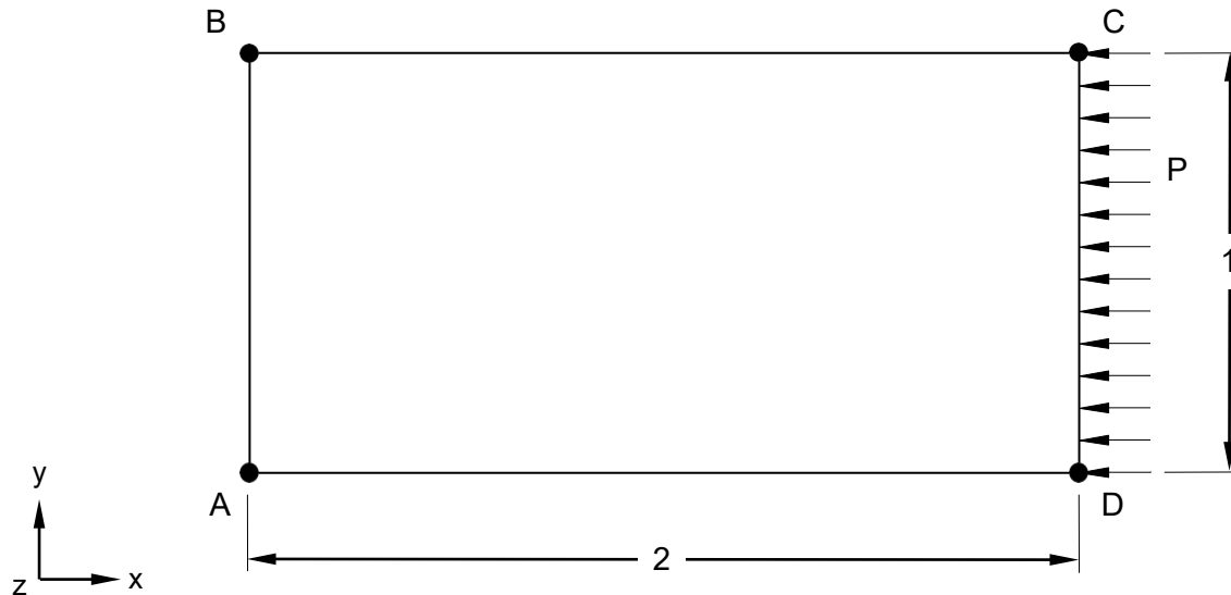
Figure 1. Plate Model
