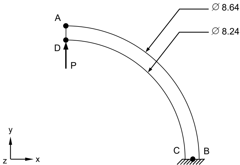
Figure 1. Beam Model
