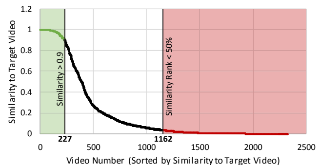
Figure 4. Similarity between a video and all other videos. We selected similar videos from the green shaded area, and dissimilar videos from the red shaded area.
