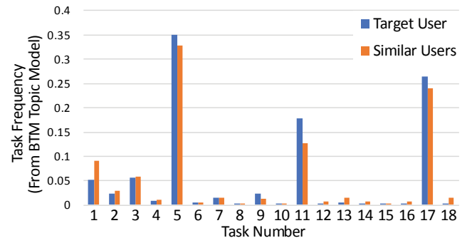
Figure 6. Example task distribution, user vs. similar users.
