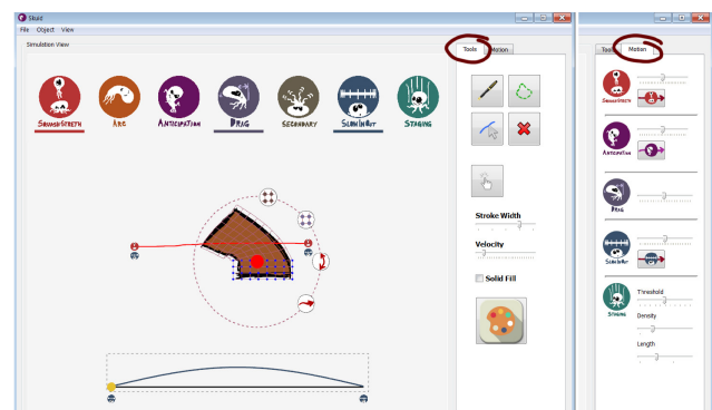
Figure 7: The system interface comprising the main canvas and the global toolbar for drawing tools (left) and motion amplifier control tools (right). Three amplifiers are in effect for the selected object.
