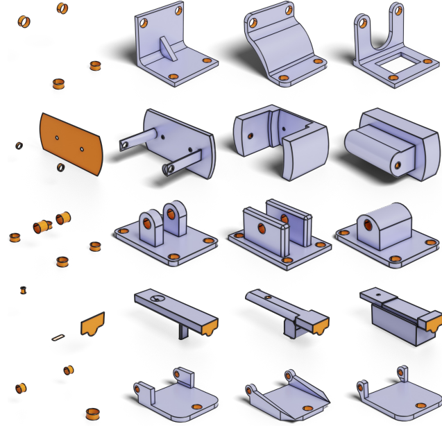
Fig. 6. Autocompletions from faces representing the assembly interfaces (orange), showing that a wide variety of shapes and styles can be generated.
