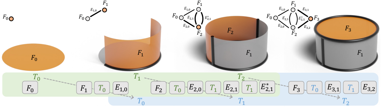
Fig. 3. Top row: Sequence ordering follows a breadth-first traversal (BFT) of the B-Rep face adjacency graph (top-left). A new face (orange) and the connecting edge(s) are added incrementally during traversal. Previously visited faces are colored in gray. Bottom row: Unified discrete tokens include face geometry F , edge geometry E , and topology reference token T for the face-edge incidence. T is dynamically assigned to every face within a local context window for unique face references. This local window corresponds to the BFT level and is updated when traversal proceeds to the next window (from green to blue). * indicates the two vertical edges connecting the same set of semi-cylindrical faces.
