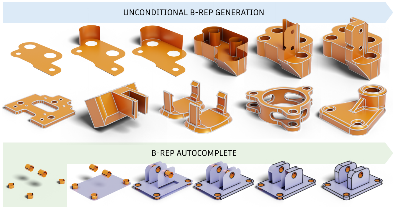
Fig. 1. AutoBrep is a single autoregressive Transformer that progressively generates B-Rep geometry and topology following a breadth-first traversal of the face adjacency graph. The model inherently supports B-Rep autocompletion, guaranteeing that the output geometry faithfully preserves the conditional faces.
