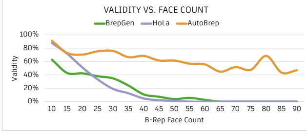
Fig. 5. Validity of generated B-Reps as a function of the face count.
