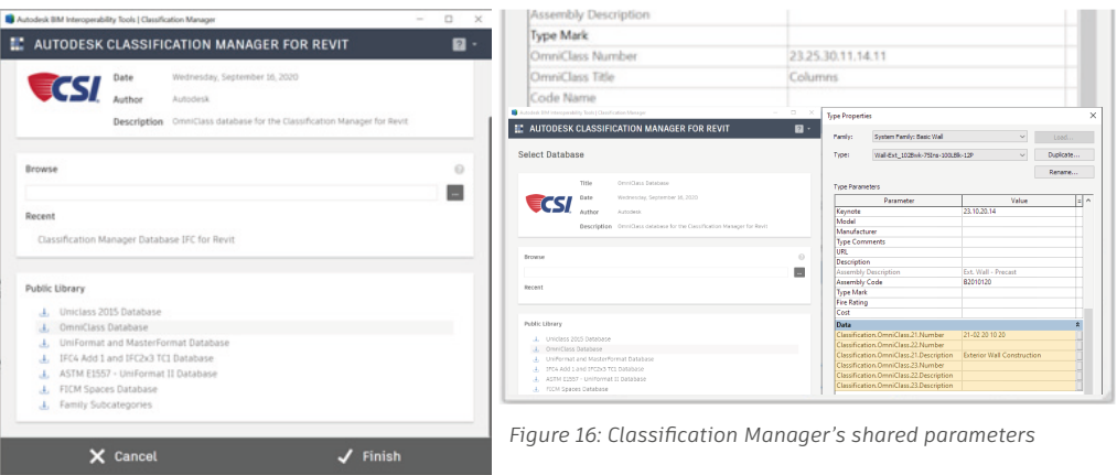
Figure 15: Revit Classification Manager
